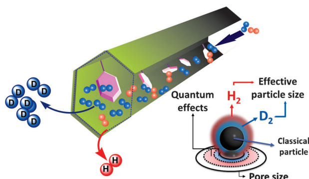
Figure 1. View of the pore channel of COF-1 with dangling pyridine molecules incorporated in the pore walls. The decreased size and the cryogenic flexibility of the aperture are employed for the enhancement of the quantum sieving effect for light isotopes.
